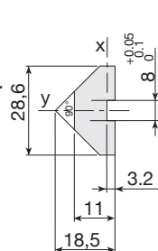
V-shaped guide rail 28.6x11
