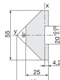
V-shaped guide rail 55x25
