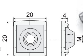
Plastic compound spring
